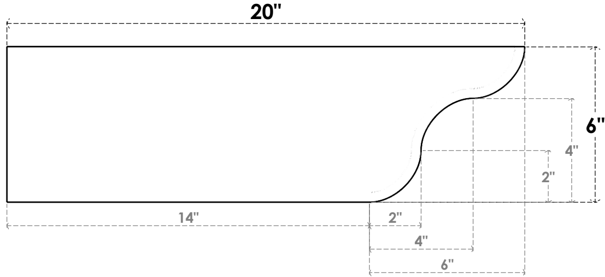
SIDE PROFILE
